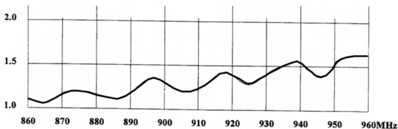
VSWR v Freq (MHz)
